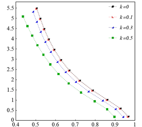
Figure 1: QNMs in the real/(negative)imaginary-plane for Schwarzschild ( k=0 ) and regular BHs with various k .
