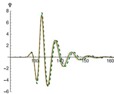
Figure 2: Gravity waveforms in the time/displacement-plane for Schwarzschild ( k=0 ) and regular BHs with various k .
