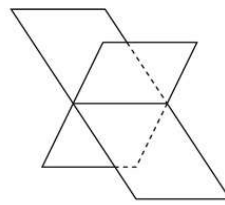
Intersecting planes
