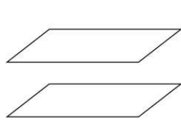
Parallel planes
